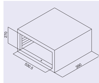
Oven Dimension GN 1/1
