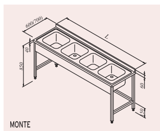
Four bowls sink unit with under shelf and fascia
