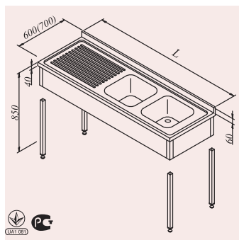
Double bowl, single drainer sink unit with fascia
