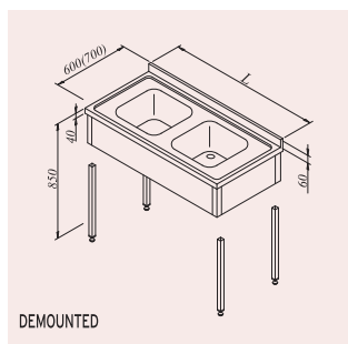
Double bowl sink unit with fascia
