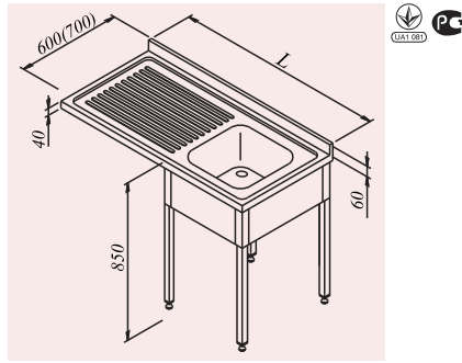
Single bowl, single drainer sink unit for dishwashing machine (square leg)
