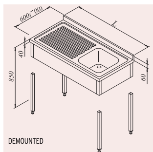
Single bowl, single drainer sink unit with fascia
