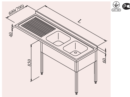
double bowl, single drainer sink unit for dishwashing machine (square leg)
