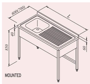
Single bowl, single drainer sink unit with under shelf and fascia
