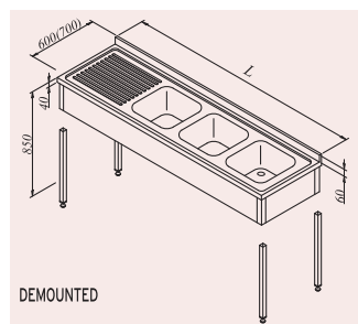
Three bowls, single drainer sink unit with fascia
