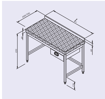
Working bench with wooden top and drawer
