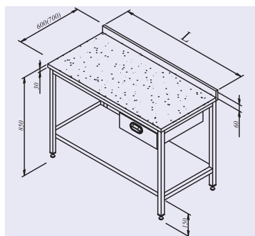
Working bench with marble top and drawer
