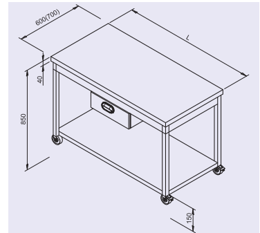
Mobile bench with drawer and shelf
