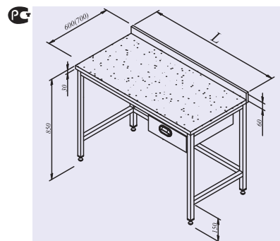
Working bench with marble top and drawer
