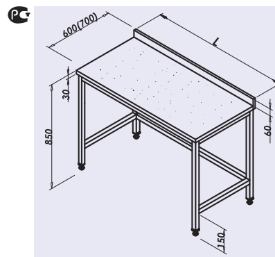
Working bench with marble top
