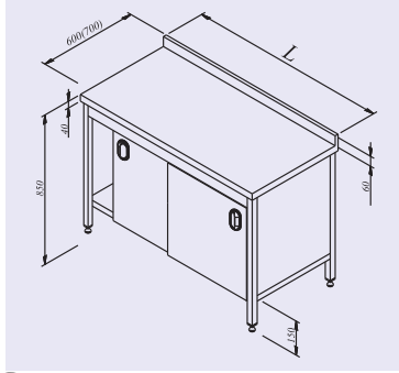
Working bench with cupboard
