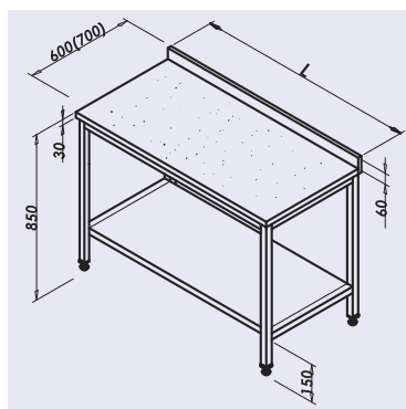
Working bench with marble top and shelf
