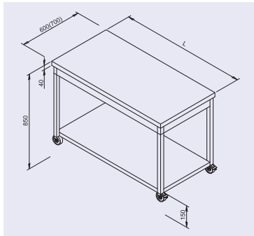
Mobile bench with shelf
