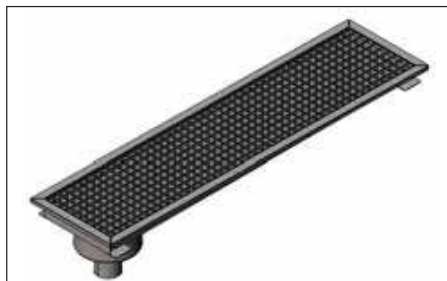
Side Drain Ø 100 Bottom Outlet
