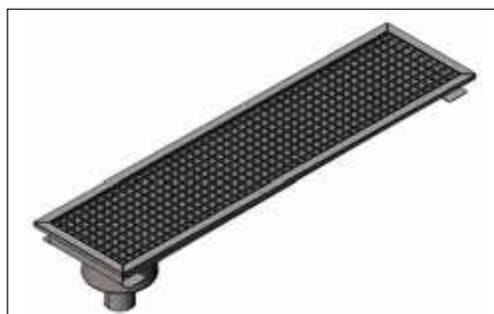
Side Drain Ø 70 Bottom Outlet
